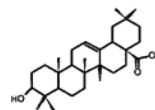
oleanolic acid 0.1-2% (w/w)
