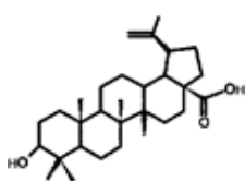
betulinic acid 0.5-6% (w/w)
